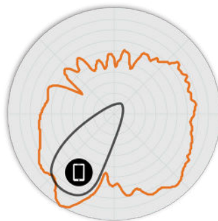
Figure 6. R770 5GHz Elevation Antenna Patterns
