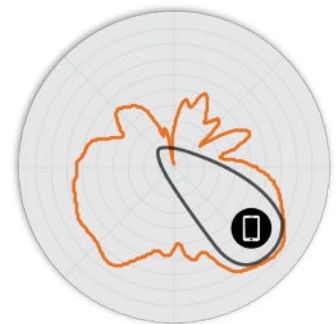
Figure 7. R770 6GHz Elevation Antenna Patterns
