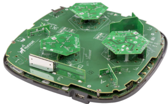
RUCKUS BeamFlex® Smart Adaptive Antenna
