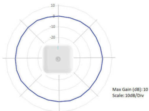
4x4 5 GHz Azimuth
