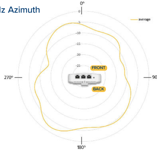
5 GHz Azimuth
