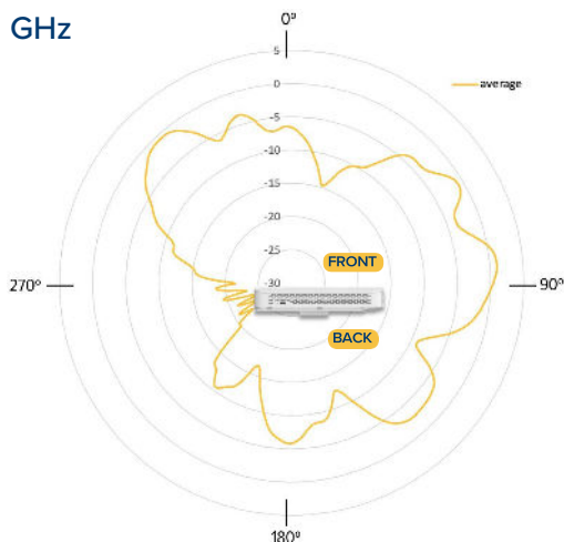
5 GHz Elevation
