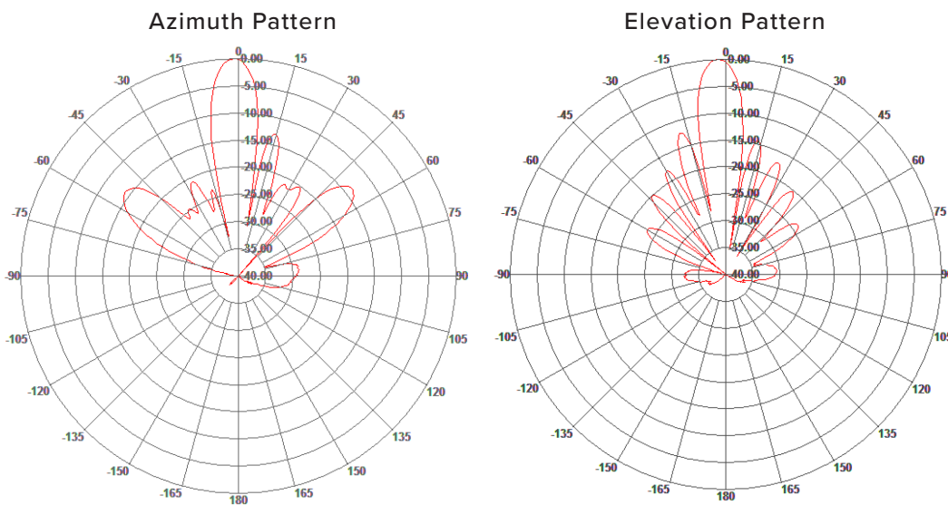
Horizontal Polarization
